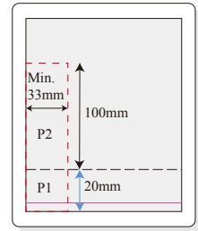
Figure 1. Cutting a sample for testing
